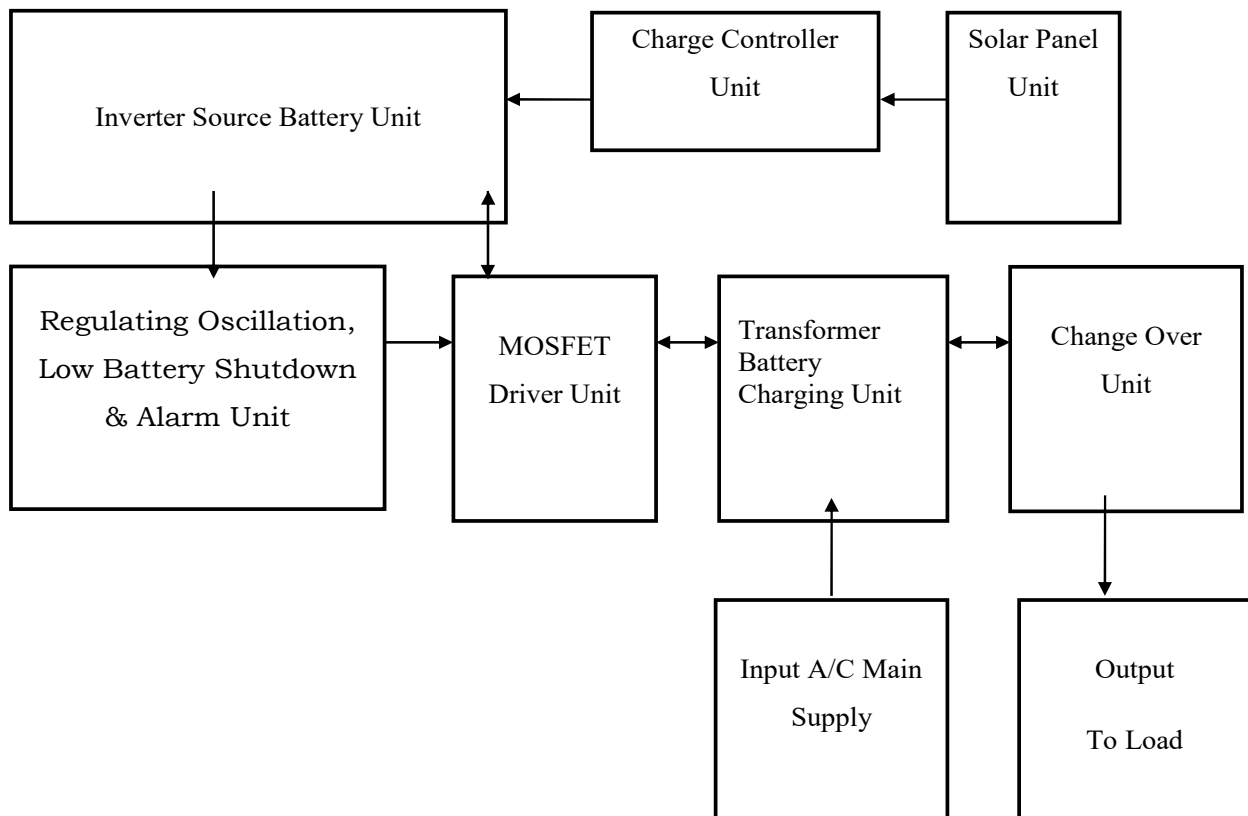
Figure 3.1: Solar power supply system block diagram
