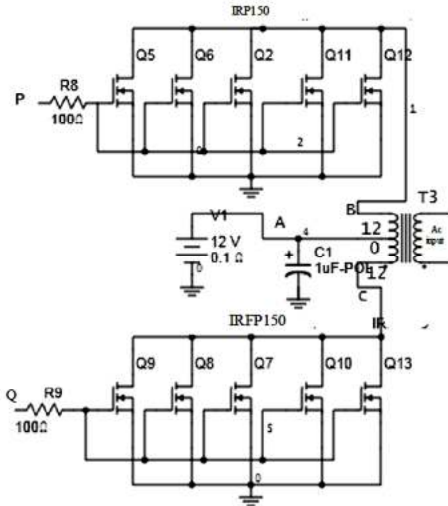
Figure 3.4 Designed MOSFET circuit in the reverse direction
